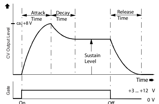
ADSR Envelope and its Parameters
