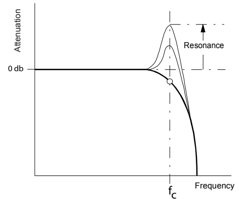
Resonance changes the filter characteristics
