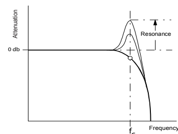
The resonance characteristics of a lowpass filter
