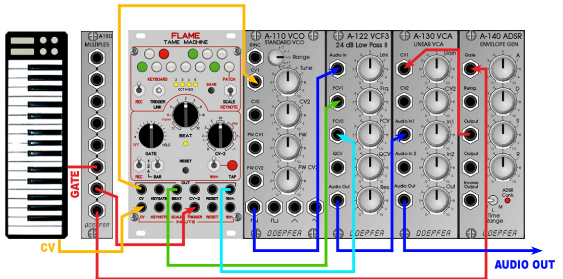
Manually playable pulsative low-pass-filter (inclusive note quantizing)
