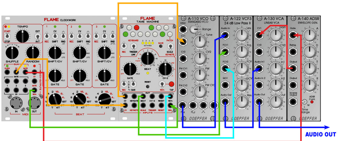
Quantizing of CV-sequences (inclusive pulsative low-pass-filter)
